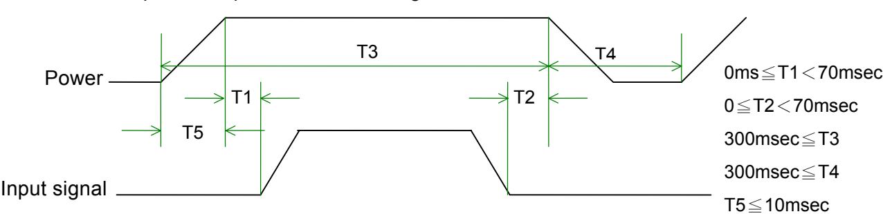
Sequence of power-on/off and signal-on/off
