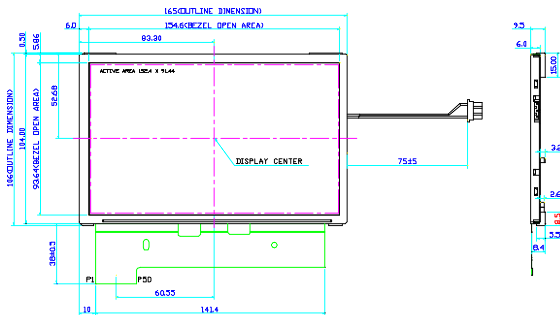
Fig.1 Outline dimension of TFT-LCD module(Front side)
